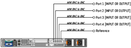
WorkflowLabs NITRO 1400 Server rearview
