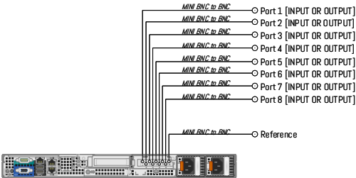
WorkflowLabs NITRO 1800 Server rearview
