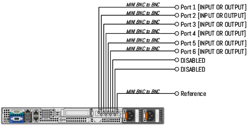
WorkflowLabs NITRO 1600 Server rearview
